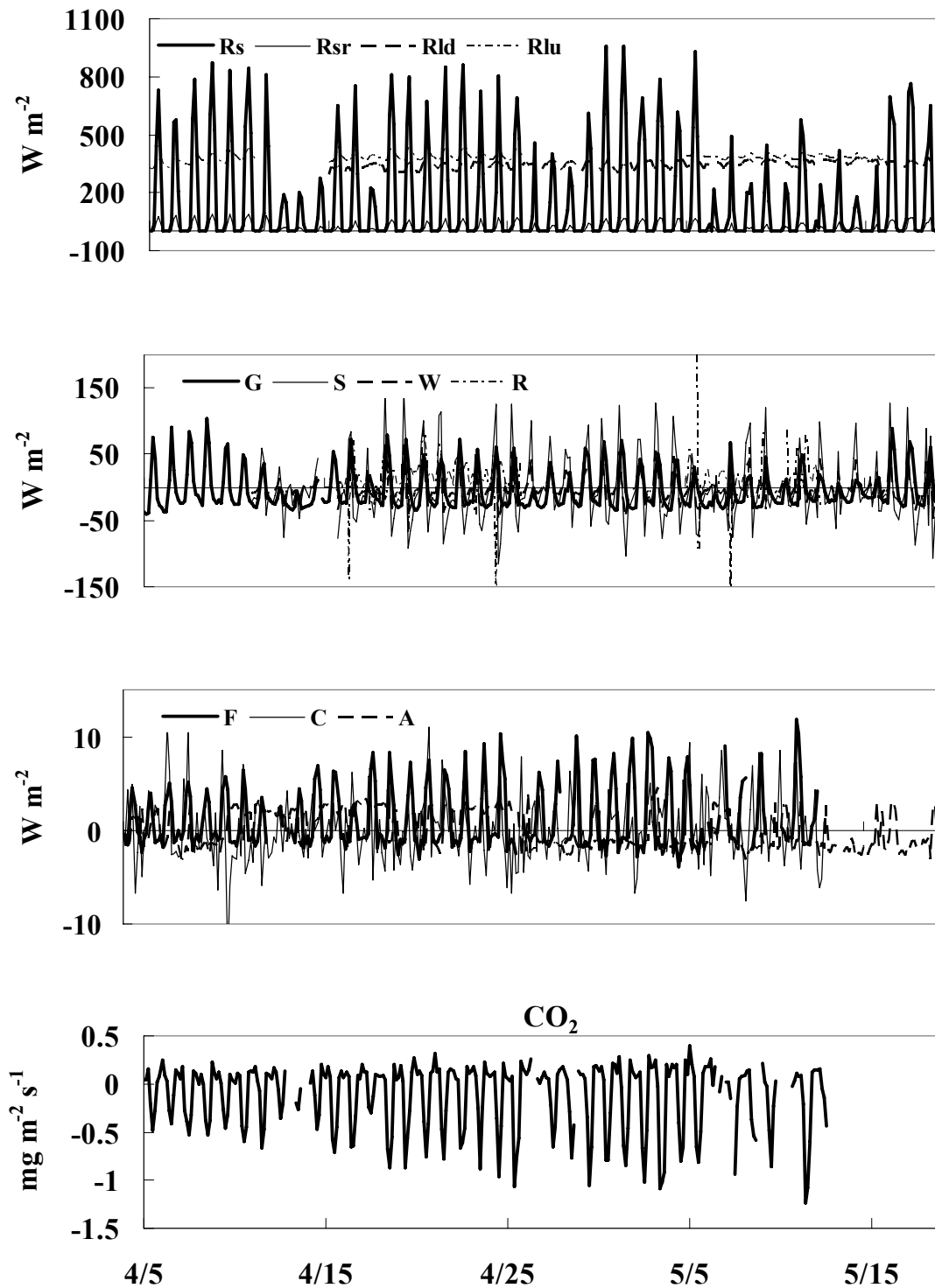
Figure 1. Net radiation ( R_n ), sensible heat flux at the canopy height ( H_c ), latent heat flux at the canopy height ( LE_c ), incoming solar radiation ( R_s ); reflected solar radiation ( R_{sr} ); atmospheric longwave radiation ( R_{ld} ); terrestrial longwave radiation ( R_{lu} ); ground heat flux ( G ), soil heat storage ( S ), liquid water heat storage ( W ), photosynthesis heat flux ( F ), canopy heat storage ( C ), advected heat flux ( A ), Residual ( R ) and CO_2 flux measured at a rice paddy site in Taiwan from
